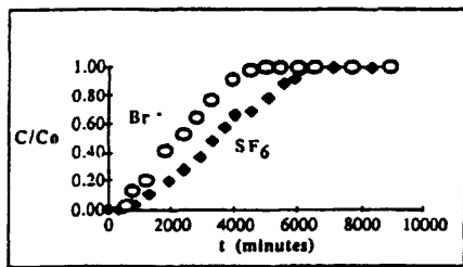
Figure 4. Breakthrough curves of Br- (empty polygons) and SF 6 (filled polygons) as observed at the pumped drain tile. Concentrations of each tracer measured (C) are relative to the steady-state concentration in the pond (C 0 ). See Figure 2 for the location of the pumping well.
